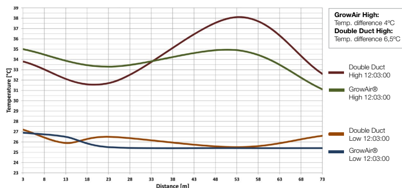
Temperature difference in the length of a duct
